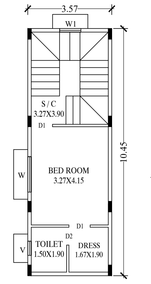
PROPOSED TYPICAL FIRST & SECOND FLOOR PLAN
