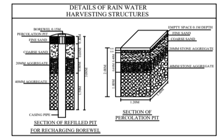
DETAILS OF RAIN WATER HARVESTING STRUCTURE
